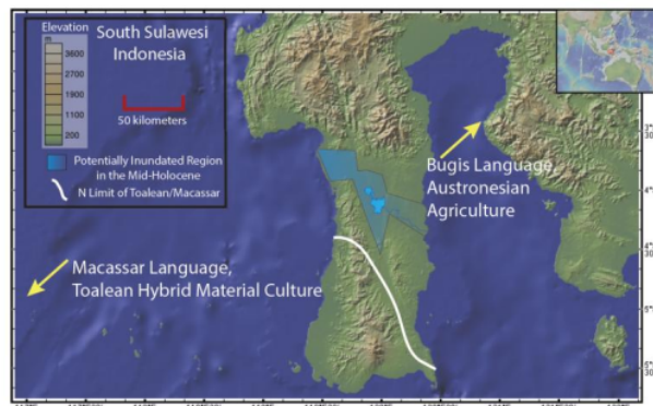
Figure 2. Physiography of South Sulawesi showing depression trending southeast through Tempe Lake. (from: Bulbeck et al., [9]).
