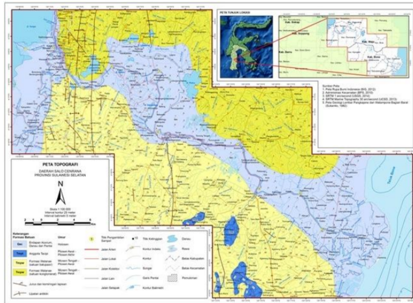
Figure 5. Geographical dan lithological map of Cenrana River.
