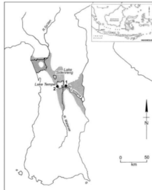
Figure 1. The estimated boundaries of formerly was sea water connecting Bone Bay in the east and Makassar Strait in the west [5].
