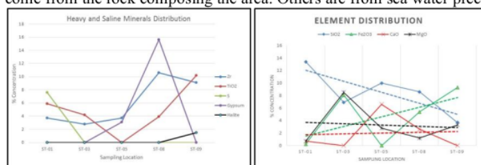
Figure 4. Concentration of element and saline minerals along the Cenrana River.
